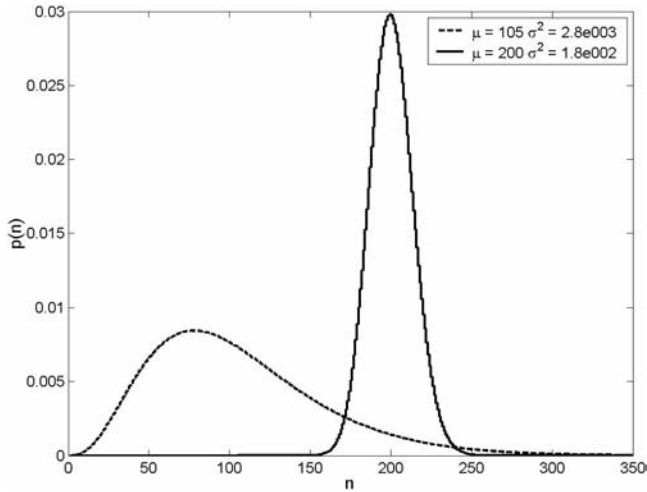
Figure 3. Two discretized gamma distributions with different means and variances. The parameters represent a decision maker's estimate of n_1 and his or her confidence in that estimate.
